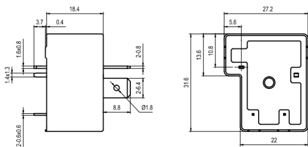
1C Outline Dimensions
