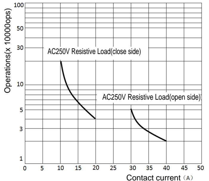
ENDURANCE CURVE
