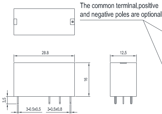
1C5 Outline Dimensions (double coils latching)
