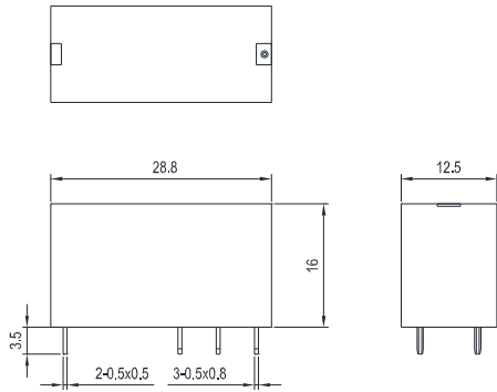
1C5 Outline Dimensions (double coils latching)
