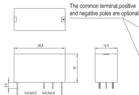
1C2 Outline Dimensions (double coils latching)
