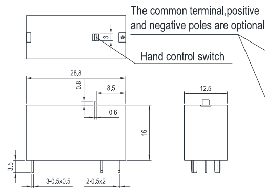
1A2/1B2 Outline Dimensions (single coil latching)
