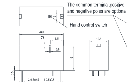
1A2/1B2 Outline Dimensions (double coils latching)
