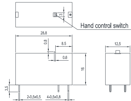
1A2/1B2 Outline Dimensions (double coils latching)
